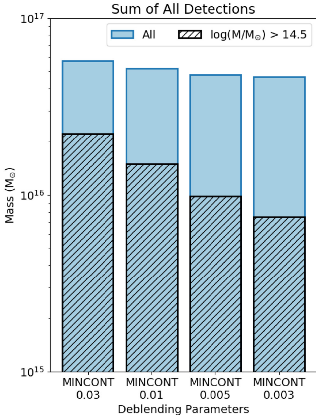
Figure 2. We plot the total mass of all overdensity candidates we find while varying the SExtractor deblending parameter DEBLEND_MINCONT . The deblending becomes finer for smaller values of DEBLEND_MINCONT . Following our expectations, finer deblending yields more low-mass overdensity candidates as more high-mass structures are broken up. Between the DEBLEND_MINCONT extremes plotted, the total mass decreases by 19 per cent, while the fraction of high-mass candidates drops by 66 per cent.
