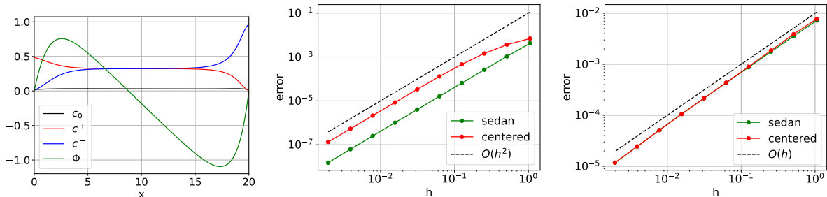
FIGURE 6. Left: stationary solution of Dirichlet problem. Center and right: results of numerical convergence test.
