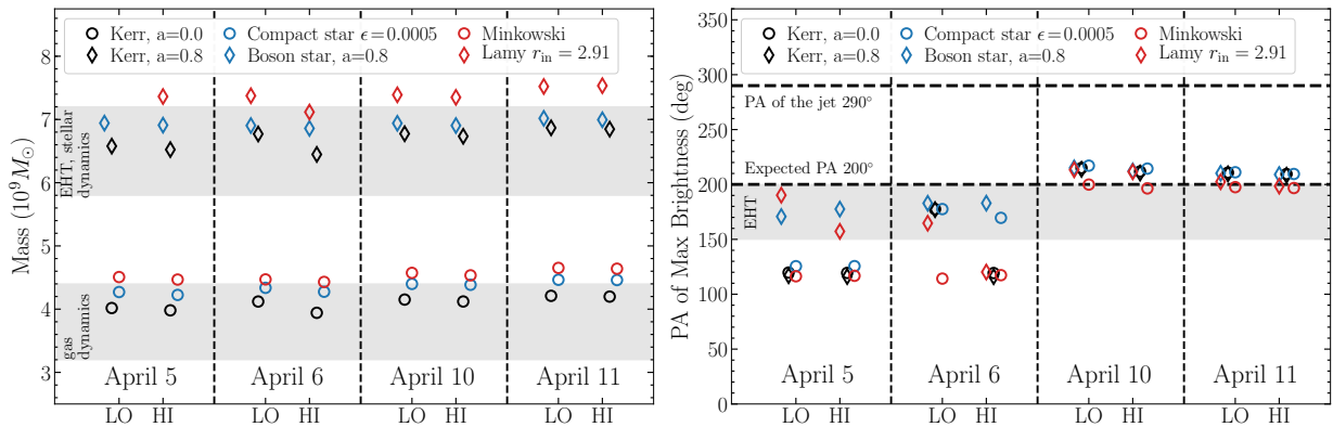
Fig. 14. Results of fitting the models of Sect. 3 to the EHT data sets. Gray bands denote previous measurements of mass and orientation of the M87*. Left: masses of the best-fit models. Different models with spin a = 0.8 give mass measurement consistent with that reported by the EHT. Models with zero spin give systematically inconsistent mass estimate. Right: position angles (east of north) of the brightest region in the best-fit models. All models constrain the brightness maximum to be located in the south of the source image, consistent with the EHT results.
