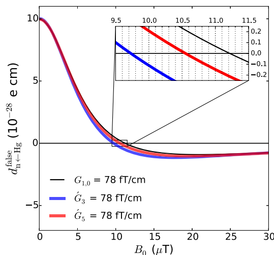
Fig. 12 False EDM due to a uniform field gradient (black), a 3-phantom mode (blue), a 5-phantom mode (red) as a function of the magnitude of the B_0 field for R = 40 \text{ cm} , H = 12 \text{ cm} , H' = 18 \text{ cm}
