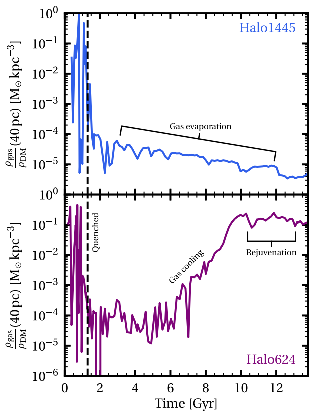
Figure 5. Evolution of the inner gas-to-dark matter density ratio at 40 pc ( \rho_{\text{gas}}/\rho_{\text{DM}} ) for two representative EDGE dwarfs. Prior to quenching by reionization (black dashed line), there are large fluctuations in \rho_{\text{gas}}/\rho_{\text{DM}} caused by repeated cycles of gas cooling, star formation, and stellar feedback. These fluctuations excite ‘dark matter heating’ that lowers the central dark matter density (Fig. 4). Halo1445 experiences no further star formation or dark matter heating after it quenches. By contrast, Halo624 grows in mass, accumulating cold gas, and rejuvenating its star formation after \sim 10 Gyr. Subsequent fluctuations are orders of magnitude smaller than at early times, and so there is no late time dark matter heating.
