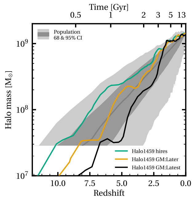
Figure 6. The halo mass growth history of Halo1459 and two modified variants which we call Halo1459 GM:Later and Halo1459 GM:Latest. Included are grey bands indicating the 68 and 95 per cent scatter for the mass growth histories of haloes throughout our lower resolution void simulation. The bands are truncated at \sim 3 \times 10^7 due to the resolution limit of the void simulation. This shows that our modified haloes are within the expected scatter of assembly histories in \Lambda CDM.
