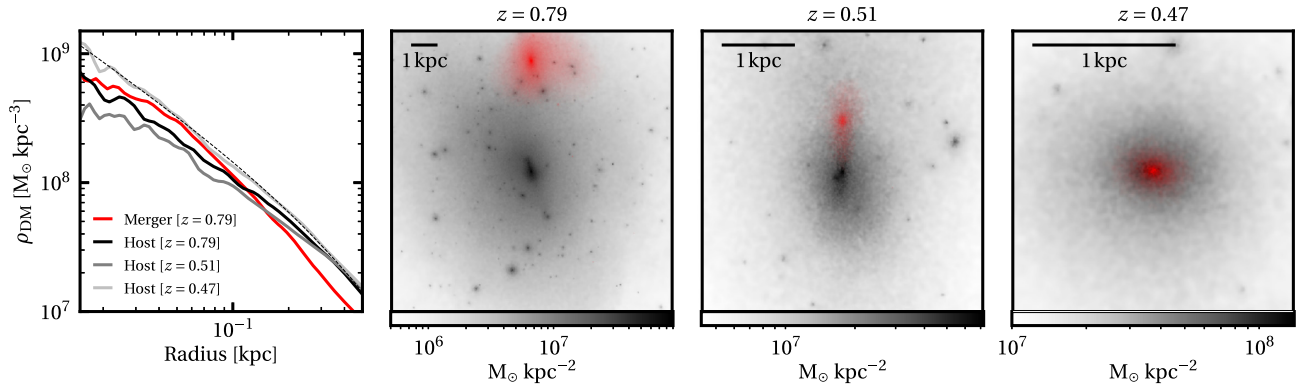
Figure 9. This plot illustrates how the reintroduction of denser dark matter material to the Halo1459 GM:Latest simulation erases the effect of earlier dark matter heating. Left-most panel: The central 3D dark matter density profiles of a cuspy subhalo (red line) and of the parent halo evolution (black, dark grey and light grey lines). The density profile of the host at z = 0.51 is centred on only the host particles to avoid any bias due to the merger. Removing the merger particles from the density profile calculation does not qualitatively change the results. A black dashed line represents a NFW profile fit to the parent halo at z = 0.79 (Navarro et al. 1997). Right-hand panels: The evolution of the merger system shown in three panels, where the parent halo is in grey-scale and the merging halo is red. The merging halo has permanently fallen into the central 100 pc of the parent halo by z = 0.47 . In all cases, the merger system has been oriented such that the centres of both haloes are in the xy -plane.
