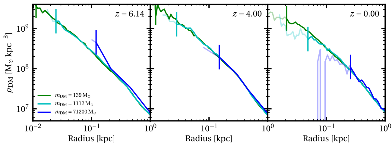
Figure A1. The evolution of the 3D density profiles for Halo1459 DMO at three dark matter particle resolutions, as stated in the legend. The two lowest particle masses (green and cyan lines) correspond to the high resolution and fiducial resolutions, respectively (see Table 1). The fainter lines indicate the radii within which at least one relaxation time (estimated using equation A1) has passed, with the transition marked using an additional vertical line for clarity. In some cases, the density profiles are not plotted at smaller radii because there are insufficient particles.
