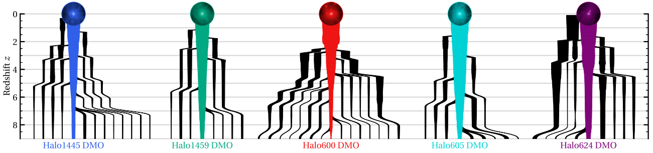
Figure 3. The accretion history of each halo as taken from the ‘DMO’ simulations, where <1/30 mass ratio mergers and sub-mergers are excluded for clarity. The central coloured branch is the main progenitor halo and the line thickness represents the M_{200c} mass of each dark matter halo.
