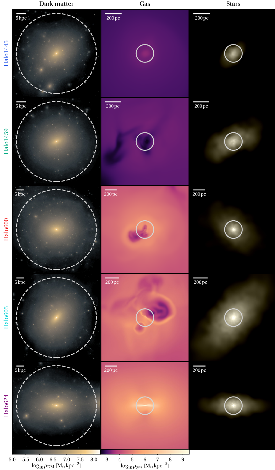
Figure 2. A visual representation of the high-resolution baryonic simulations in Table 1. Left-hand panels: The dark matter surface density out to r_{200c} (dashed circle). Middle panels: The gas density averaged along a 0.2 kpc slice through z . The 3D half-light radius is indicated by the solid circle. Right-hand panels: The halo stars are rendered in PYNBODY with the i , v , and u bands over the range 23 \leq \text{mag arcsec}^{-2} \leq 28 , shown at the same scale as the gas density panels. All images are oriented side-on along the angular momentum vector of the cool gas ( < 10^4 K) within 1 kpc of the halo centre. The physical size of each frame is indicated by a scale bar in the top left corner.
