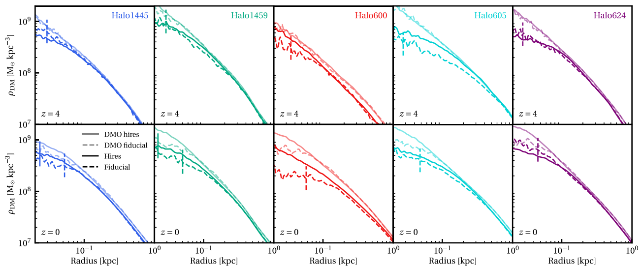
Figure B2. The 3D dark matter density profiles of our main simulation suite, where we compare our DMO simulations (faint lines) and baryonic simulations (opaque lines) at fiducial (dashed lines) and high (solid lines) resolution. The upper panels show this comparison at z = 4 , by which time all haloes are quenched due to reionization (some will later reignite their star formation). The lower panels show this comparison at z = 0 . The numerical relaxation radius, as defined in Appendix A, is indicated by a short vertical line for the baryonic simulations. This limit is similar for the corresponding DMO simulations.
