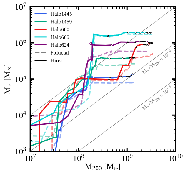
Figure B1. The stellar mass–halo mass relation through time for our main simulation suite, where we compare our fiducial resolution simulations (faint dashed lines) to our high-resolution simulations (solid lines). The black circles on the high-resolution lines mark intervals of 1 Gyr in time. The grey diagonal lines show constant ratios of M_*/M_{200c} in powers of 10, as marked.
