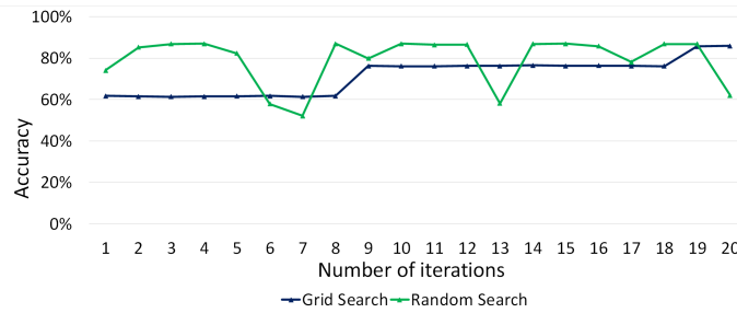
Fig. 8. Comparison between two hyper-parameter tuning approaches
