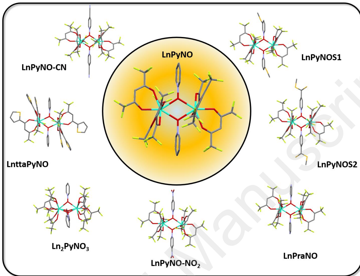
Figure 1. Representation of the dimers LnPyNO , 1,4 LnPyNOS1 , 40 LnPyNOS2 , 40 LnnttaPyNO , 2 Ln 2 PyNO 3 , 41 LnPyNO-NO 2 , 3 LnPraNO , 5 together with LnPyNO-CN 38 the seminal dimer that inspired the study; see text for abbreviations.
