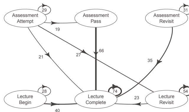
Fig. 1. Transition graph of interactions with course content for all learners. Interaction states are defined by content type and progress level (cf. Table 2). Arrow thickness is proportionate to transition probability, which is provided as percentages next to the arrowhead. Only showing arrows for probabilities above 15%.
