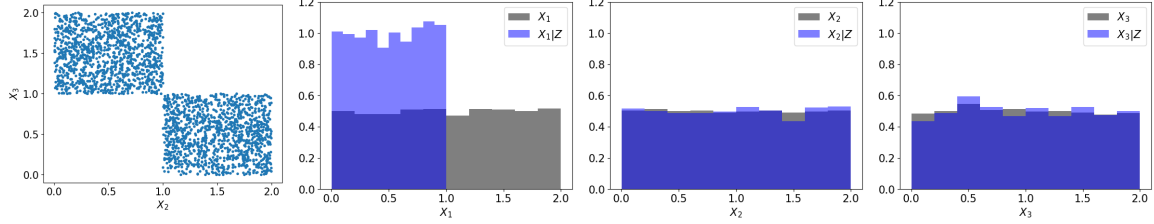
Figure 3: From left to right: 1 - Pairs of (X_2|Z = 1, X_3|Z = 1) . 2 - Histogram of X_1 and X_1|Z = 1 . 3 - Histogram of X_2 and X_2|Z = 1 . 4 - Histogram of X_3 and X_3|Z = 1 .
