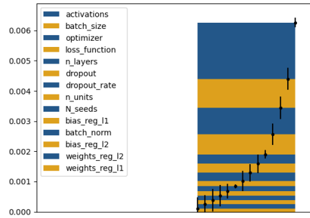
Figure 14: HSICs for \mathcal{G}_{\text{dropout\_rate}} of MNIST hyperparameter analysis. Conditional hyperparameter dropout_rate is not impactful.
