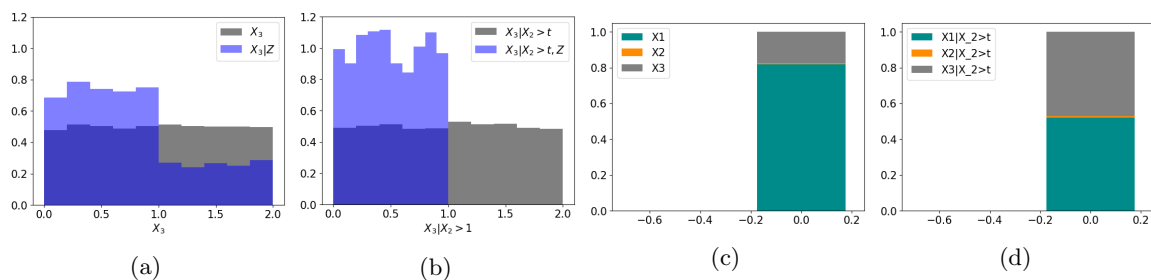
Figure 6: (a) - Histogram of X_3 and X_3|Z (b) - Histogram of X_3 and X_3|X_2 > t, Z . (c) - S_{X, \mathbf{Y}} for X_1 ; X_2 and X_3 . (d) - S_{X, \mathbf{Y}} for X_1|X_2 > t ; X_2|X_2 > t and X_3|X_2 > t .
