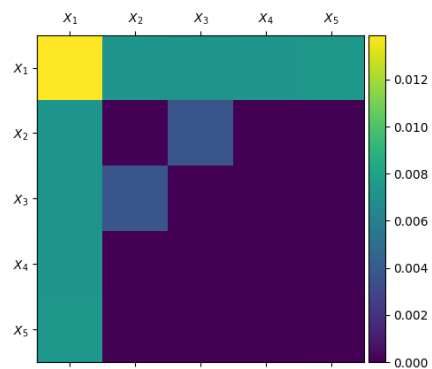
Figure 4: S_{X, \mathbf{Y}} for each pair of variable.
