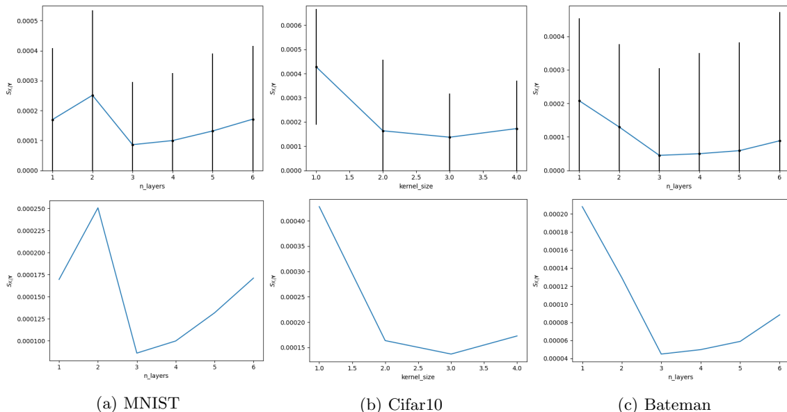
Figure 13: S_{X_i|X_i \in \{a+c, \dots, b\}, \mathbf{Y}} w.r.t. c for (a) n_layers in MNIST, (b) kernel_size in Cifar10 and (c) n_layers in Bateman with error bars ( top ) and without error bars ( bottom ). The error bars traduce the standard estimation error.
