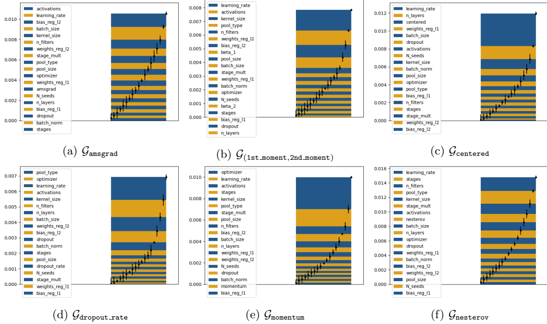
Figure 16: HSICs for conditional groups of cifar10 hyperparameter analysis. (a): amsgrad is not impactful, (b): 1st_moment , 2nd_moment are not impactful, (c): centered is the third most impactful hyperparameter of this group, (d): dropout_rate is not impactful, (e): momentum is not impactful, (f): nesterov is not impactful.
