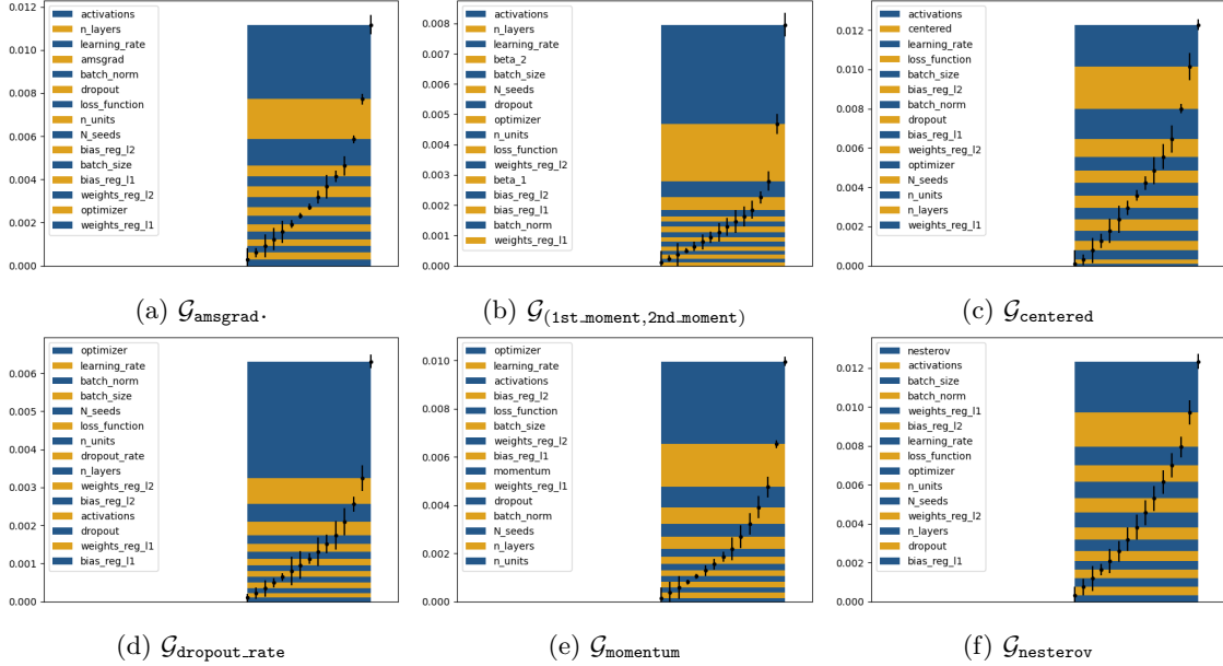
Figure 15: HSICs for conditional groups of Bateman hyperparameter analysis. (a): amsgrad is not impactful (it is in the estimation noise), (b): 1st_moment is not impactful but 2nd_moment is the fourth most impactful hyperparameter of this group, (c): centered is the second most impactful hyperparameter of this group, (d): dropout_rate is not impactful, (e): momentum is not impactful, (f): nesterov is the most impactful hyperparameter of this group.
