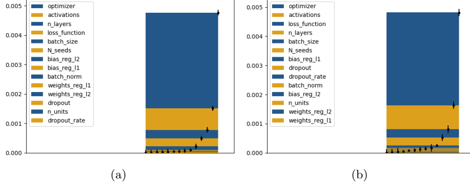
Figure 8: Comparison of S_{X_i, \mathbf{Y}} without considering conditionality (a) and for variables X_i \in \mathcal{G}_l (b)
