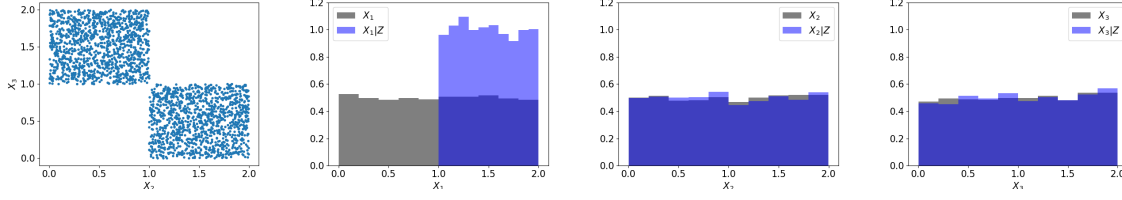
Figure 3: From left to right: 1 - Pairs of (X_2|Z = 1, X_3|Z = 1) . 2 - Histogram of X_1 and X_1|Z = 1 . 3 - Histogram of X_2 and X_2|Z = 1 . 4 - Histogram of X_3 and X_3|Z = 1 .
