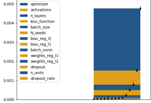
Figure 2: Comparison of S_{X_i, \mathbf{Y}} for hyperparameters in Runge approximation problem.
