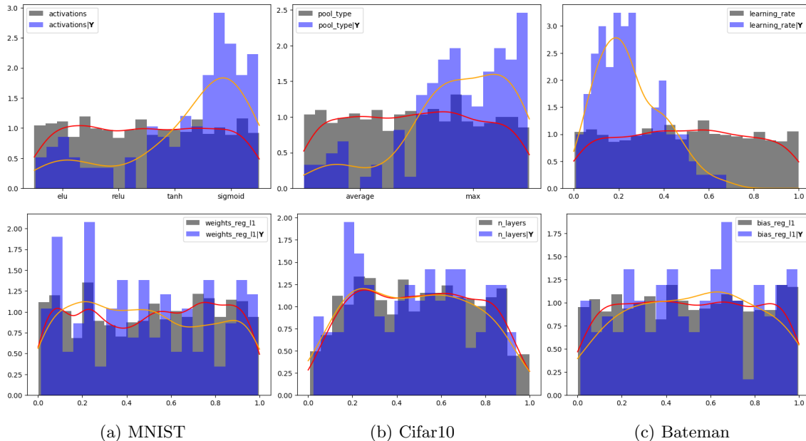
Figure 10: Representation of U_i|Z = 1 (orange for KDE and blue for histogram) and U_i (red for KDE and grey for histogram), for hyperparameters X_i with high (top) and low (bottom) S_{X_i, \mathbf{Y}}
