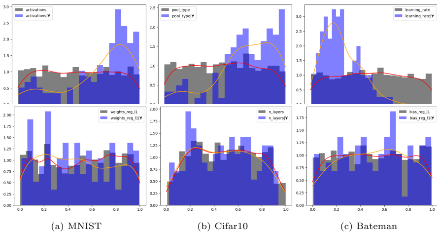
Figure 10: Representation of u_i|z = 1 (orange for KDE and blue for histogram) and u_i (red for KDE and grey for histogram), for hyperparameters x_i with high (top) and low (bottom) S_{x_i, \mathbf{Y}}
