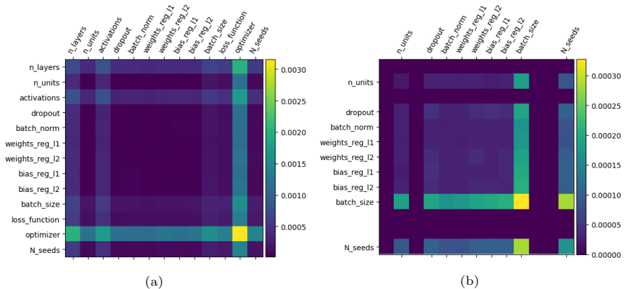
Figure 5: (a) S_{(x_i, x_j), Y} for each pair of hyperparameters. (b) S_{(x_i, x_j), Y} for each pair of hyperparameters, except for optimizer , activation , n_layers and loss_function . The grid can be read symmetrically with respect to the diagonal.
