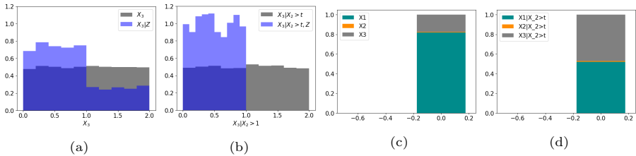
Figure 6: (a) - Histogram of x_3 and x_3|z = 1 (b) - Histogram of x_3 and x_3|x_2 > t, z . (c) - S_{x_i, \mathbf{Y}} for x_1 ; x_2 and x_3 . (d) - S_{x_i, \mathbf{Y}} for x_1|x_2 > t ; x_2|x_2 > t and x_3|x_2 > t .
