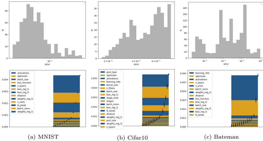
Figure 9: (top) Histograms of the initial random sampling of configurations and (bottom) comparison of S_{x_i, \mathbf{Y}} for every main hyperparameters.
