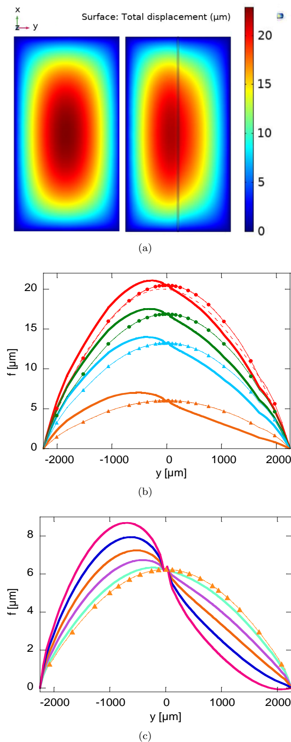
Fig. 4 Consol simulation of the deformation of the system. (a) Total surface displacement profiles on top ( z = H ) and bottom surfaces ( z = h_0 ), respectively, for \Delta P = 1620 Pa and \langle P \rangle = 3752 Pa. The position of the pad is highlighted on the right by two lines. (b) Line field displacement profiles f along y -axis for x = 0 and various values of \langle P \rangle and z . Red: \langle P \rangle = 3752 Pa, Green: \langle P \rangle = 3090 Pa, Blue: \langle P \rangle = 2428 Pa, Orange: \langle P \rangle = 1104 Pa - Dotted lines: \Delta P = 0 Pa and z = h_0 , Full lines: \Delta P = 1620 Pa and z = h_0 . Dashed line: \Delta P = 1620 Pa and z = H (c) Line field displacement profiles f along y -axis for x = 0 , z = h_0 and \langle P \rangle = 1104 Pa. Dotted Orange line: \Delta P = 0 Pa, Magenta: \Delta P = 3237 Pa, Blue: \Delta P = 2428 Pa, Full orange line: \Delta P = 1620 Pa, Purple: \Delta P = 971 Pa, Light Green: \Delta P = 324 Pa.
