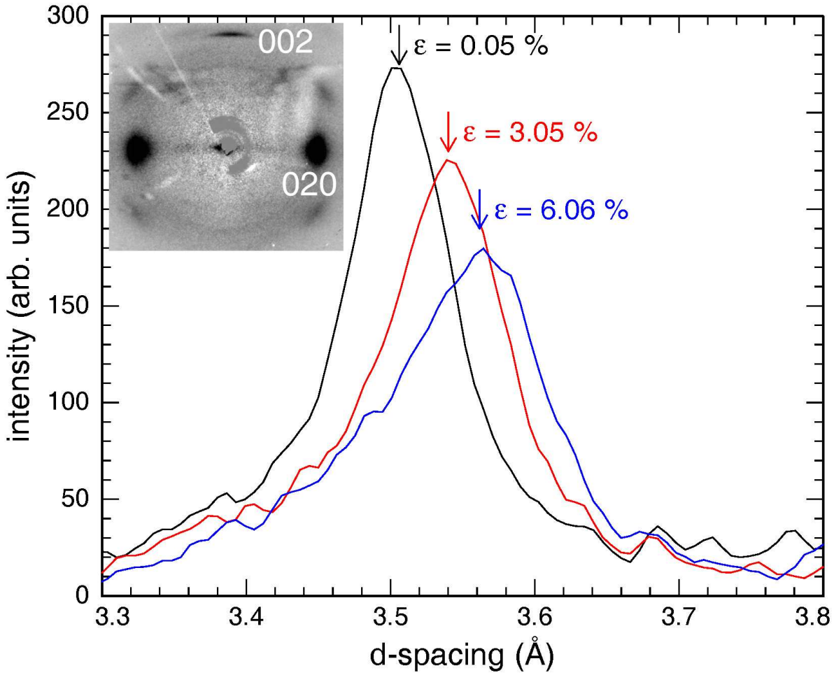
Figure 3: Results from the X-ray diffraction experiments on Bombyx silk fibers at the HASY-LAB beamline A2. The inset shows the average of all 23 two-dimensional diffraction patterns recorded after background subtraction. The inhomogeneity of the remaining background is due to the saturation in the center of the diffraction diagram, to a different shading of parts of the detector at different strain, and to the glass capillary of the beamstop holder (diagonal line to the center). The sample was tilted by the Bragg angle of the clearly visible meridional 002 reflection (indexed according to 12 ). The two strong reflections on the equator are indexed 020, the four equivalent weaker reflections 021. An azimuthal integration of the 002 reflection at different strain \epsilon leads to the curves in the main figure. The expansion of the unit cell with increasing strain in the direction of the c -axis is well visible.
