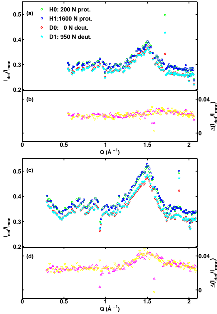
Figure 5: Diffraction patterns of Bombyx mori silk fibers obtained from the data recorded on IN6 according to equation 2, normalized to the incident beam monitor and to the total scattering according to the set of equations 4, and approximately corrected for the individual detector efficiencies by vanadium scattering. The data are plotted versus the absolute value of the total scattering vector Q . The lowest 4 detectors have been omitted. (a): Data recorded in the top detector row (inclined by 15^\circ with respect to the equatorial plane). (b): Difference patterns from the protonated and deuterated sample for the top detector bank ( \Delta -symbols: H1-D1; \nabla -symbols: H0-D0). (c) Data recorded in the equatorial plane of the fibers (middle detector row). The legend of (a) applies to (c) as well. (d): Difference patterns from the protonated and deuterated sample for the middle detector bank ( \Delta -symbols: H1-D1; \nabla -symbols: H0-D0).
