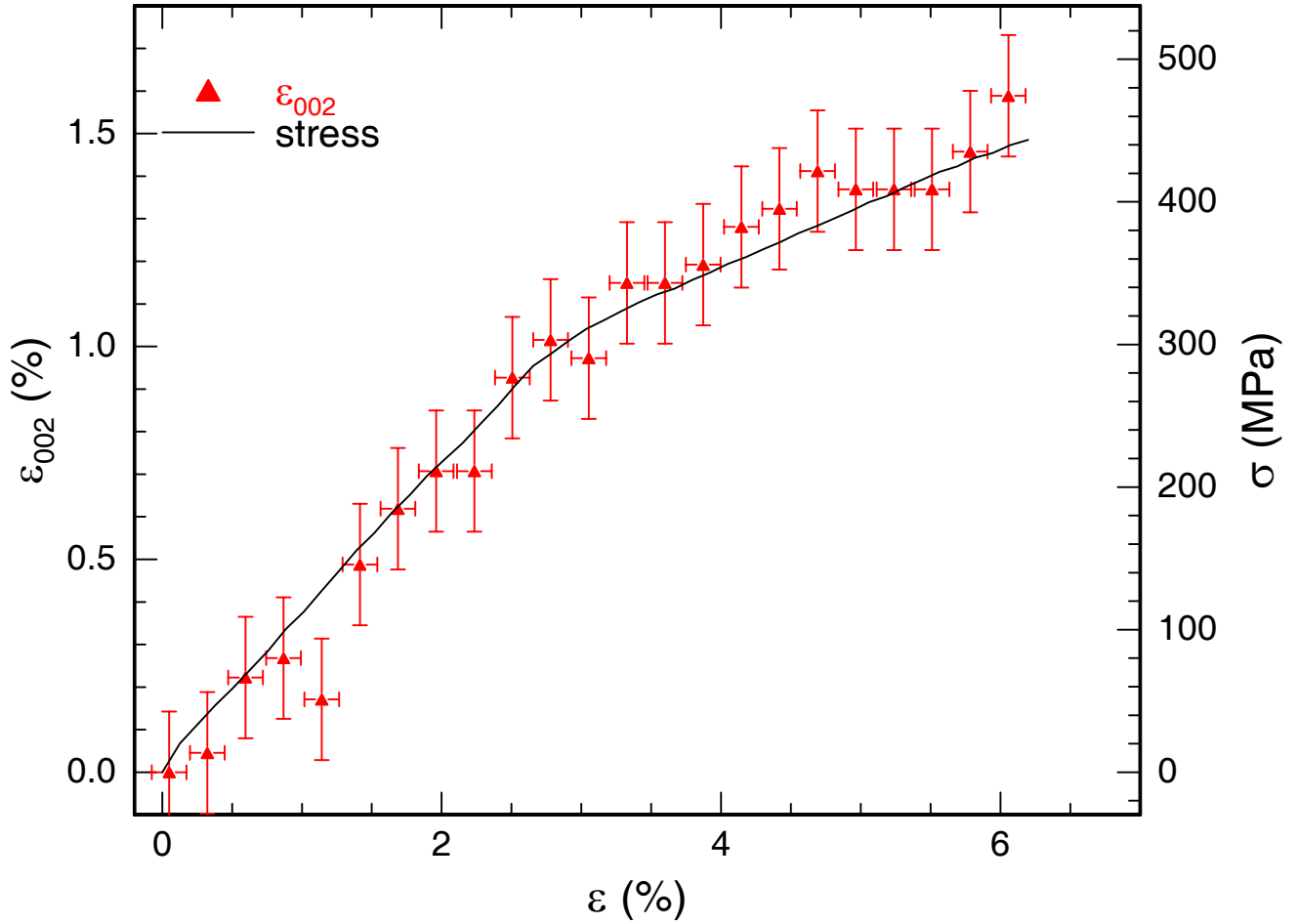
Figure 4: Crystal strain ( \epsilon_{002} ) (symbols, left y-axis) within Bombyx silk fibres as extracted from the synchrotron X-ray diffraction data (figure 3) and stress \sigma (line, right y-axis, same as the black line in figure 2) measured in-situ during this experiment, plotted versus the measured strain \epsilon of the fiber.
