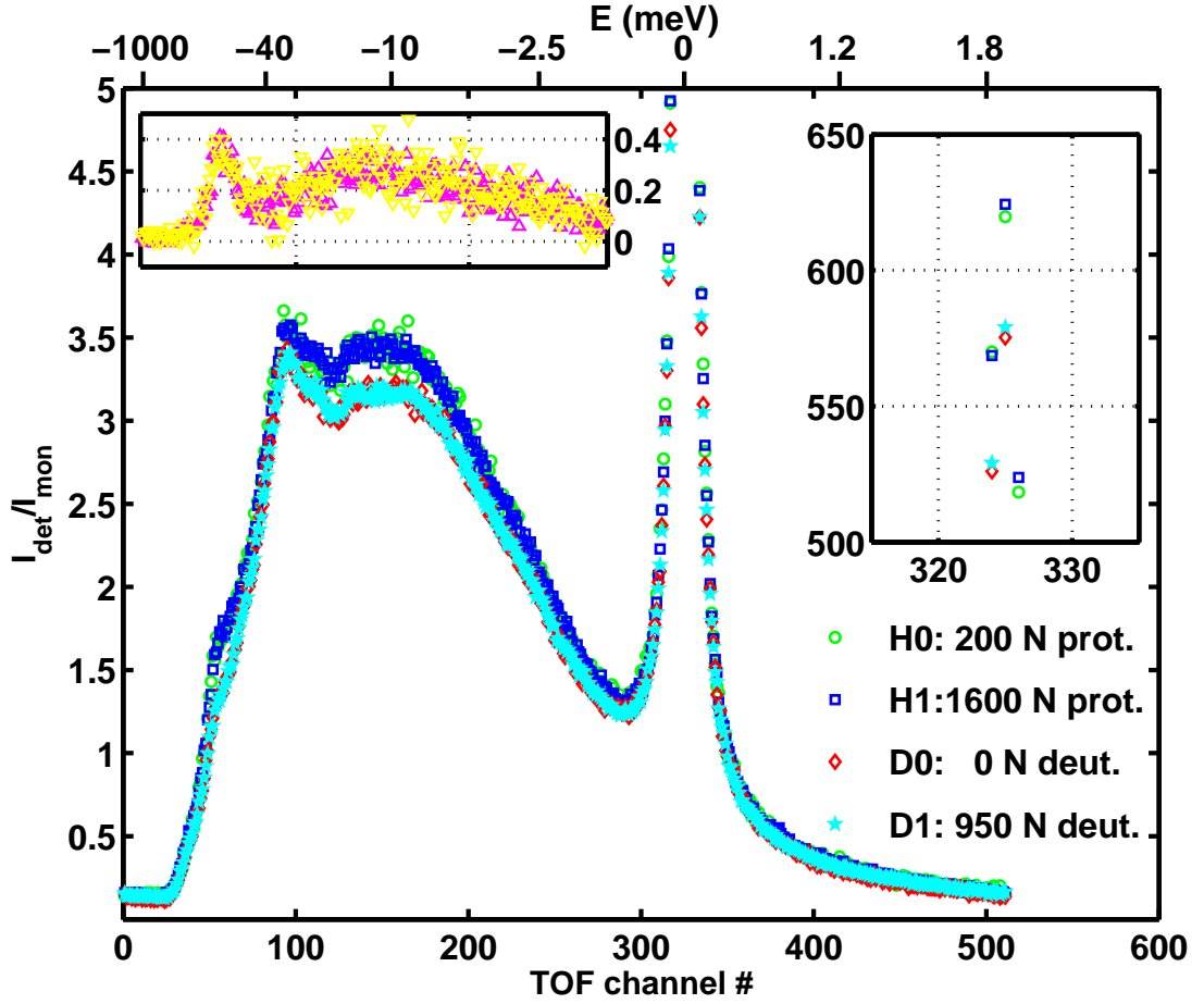
Figure 6: Time-of-flight spectra of Bombyx mori silk recorded on IN6. The intensities recorded in all detectors within the equatorial plane have been summed up. The intensities are normalized to the incident beam monitor and corrected for the change in the total illuminated sample volume due to the different extension upon the externally applied stress (see main text for further explanation). The data are plotted versus the time-of-flight channel number. The corresponding calculated energy transfer is indicated in the additional top x-axis. The elastic peak maxima are plotted in the right inset using the same axis units as in the main figure. The legend assigns the symbols for both the main part of the figure and the right inset. The difference spectra from the protonated and deuterated sample are given in the left inset. Here, the time-of-flight and energy axis are identical to the corresponding axes of the main part of the figure, and the \triangle -symbols correspond to the difference between the protonated sample at 1600 N and the deuterated sample at 950 N (H1-D1), whilst the \nabla -symbols denote the difference between the protonated sample at 200 N and the deuterated sample at 0 N (H0-D0).
