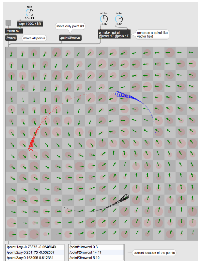
Figure 1: Graphical user interface of simone .
