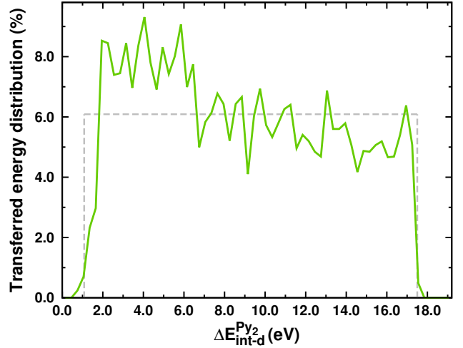
Fig. 3 Distribution of transferred energy in rovibrational modes \Delta E_{int}^{Py_2} for trajectories leading to dissociation at the end of MD (center of mass collision energy of 17.5 eV). The dashed line shows the distribution of transferred energy used in the LOC model.
