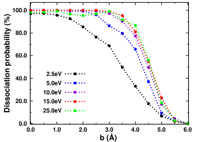
Fig. 4 Opacity curves as a function of the impact parameter b for several selected center of mass collision energies.
