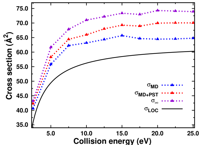
Fig. 5 Dissociation cross sections of \text{Py}_2^+ after collision with Argon as a function of center of mass collision energy for the short (MD), experimental (MD+PST) and infinite timescales. Cross sections resulting from the LOC model are also plotted.
