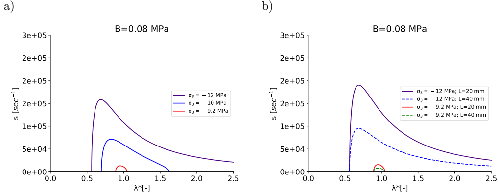
Figure 14: Growth coefficient vs the normalized perturbation wavelength under several confining pressures for B=0.08 MPa ( \rho=1600 \text{kg/m}^3 in all cases): (a) for L=24 mm; (b) Effect of the material length L .
