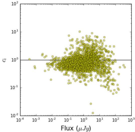
Figure 5. Covariance index c_i as a function of measured fluxes from T-PHOT for the MACS0416 cluster. 527 (16 per cent) sources from our catalogue lie above c_i > 1 and are treated with caution.
