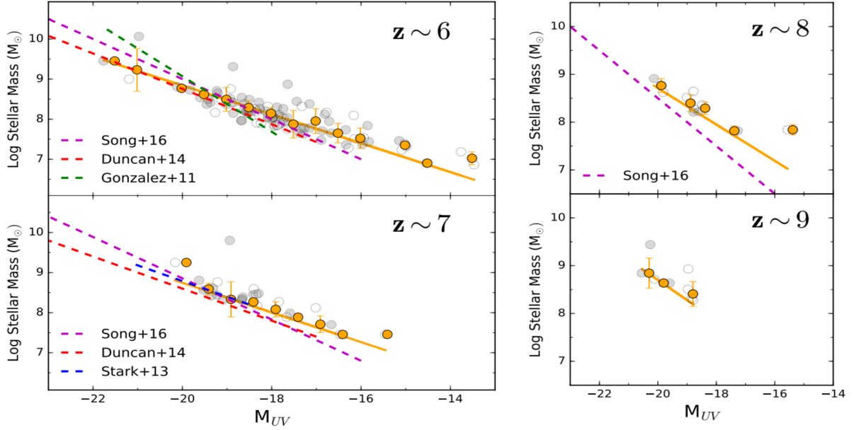
Figure 15. Stellar mass as a function of rest-frame absolute UV magnitude at 1500 \text{ \AA} at z = 6-9 . Grey filled circles represent sources with an S/N ratio > 3\sigma at 3.6 \mu\text{m} in IRAC, whereas grey open circles are those with an S/N ratio \lesssim 3\sigma . Filled yellow circles represent the median stellar masses in each rest-frame absolute UV magnitude bin of 0.5 \text{ mag} , and the yellow error bars represent the standard deviation in stellar mass in each UV magnitude bin. The best-fitting \log_{10}(M_*/M_\odot) - M_{UV} relation is shown by solid yellow line in each redshift bin. The best-fitting \log_{10}(M_*/M_\odot) - M_{UV} lines of González et al. (2011), Stark et al. (2013), Duncan et al. (2014), and Song et al. (2016) are also shown by green, blue, red, and magenta dashed lines, respectively, for comparison.
