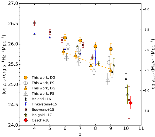
Figure 18. Evolution of UV luminosity density as a function of redshift. \rho_{UV} values calculated with an M_{UV} = -13.5 limit are shown in orange filled circles and \rho_{UV} calculated using an M_{UV} = -17 limit are shown in orange filled triangles. Also shown are the \rho_{UV} estimates considering point sources in our completeness simulations with open grey circles and open grey triangles for M_{UV} = -13.5 and M_{UV} = -17 , respectively. The literature points shown are estimated with an M_{UV} = -17 limit. The dashed yellow line is the power-law fit to the data points at z \sim 6-9 , such that \rho_{UV} \propto (1+z)^{-2.63} . Fitting a power law at z \geq 8 values results in \rho_{UV} \propto (1+z)^{-4.61} (not shown).
