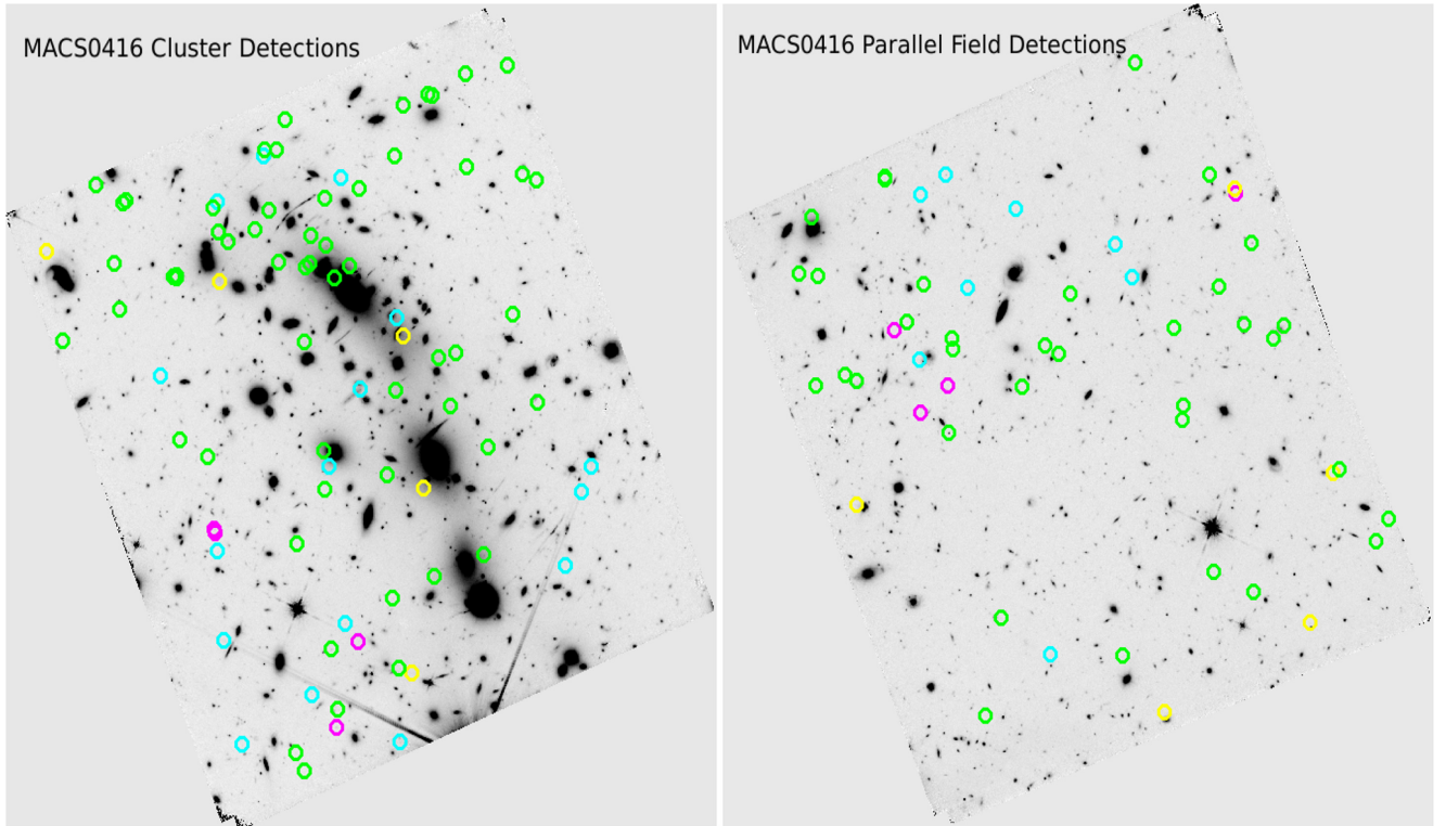
Figure 6. H -band image of the MACS0416 cluster (left) and the parallel field (right). The positions of our high- z galaxy sample at z = 6, 7, 8, and 9 are shown by green, cyan, yellow, and magenta circles, respectively.
