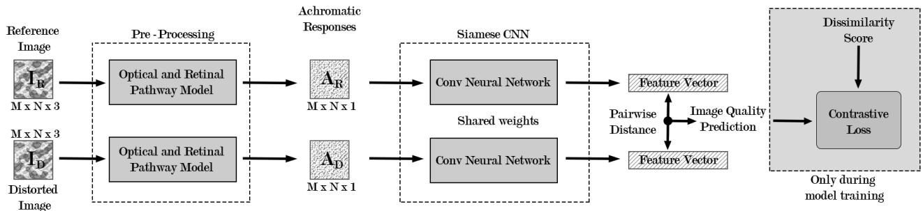
Figure 1: Diagram of the proposed model where I_{R/D} indicates the input images, and A_{R/D} denotes the achromatic responses. Reference and distorted image pairs inputted to the Siamese CNN after the pre-processing. Siamese CNN outputs is used for image quality prediction. During training, dissimilarity scores derived from MCL-JCI dataset is used for training via contrastive loss.
