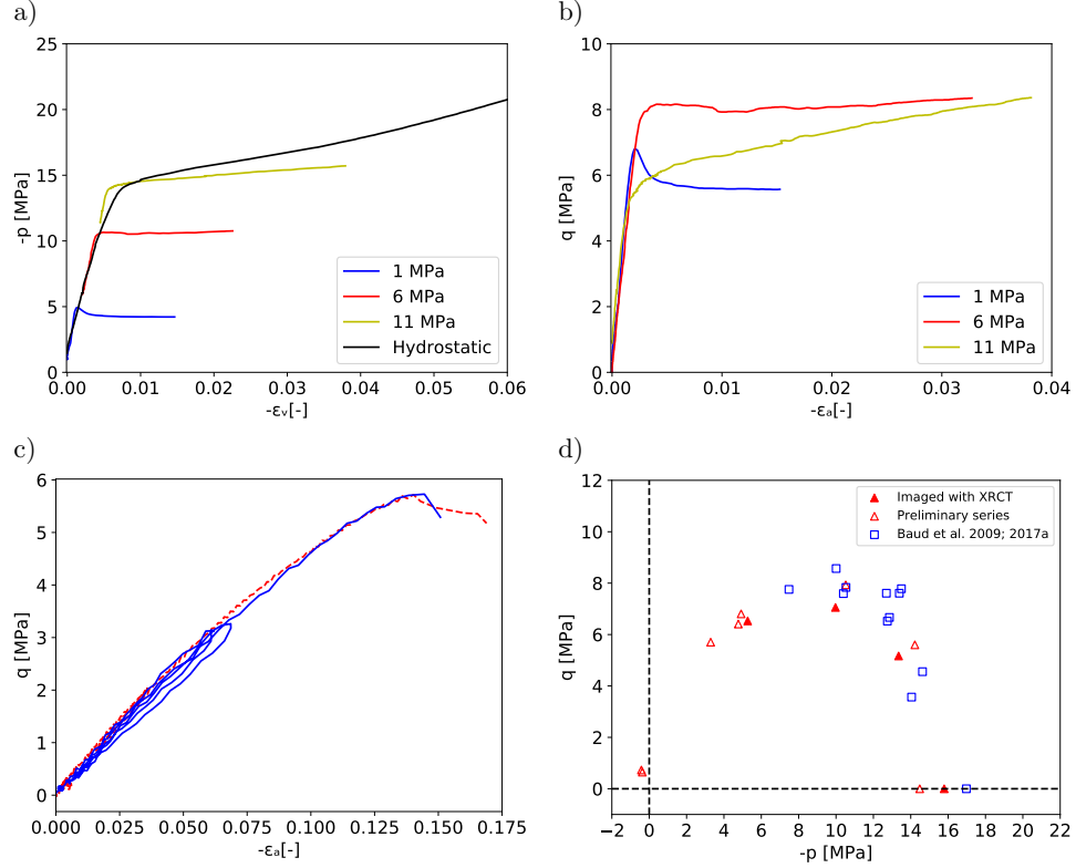
Figure 6: Mechanical reponse of the SML tested under several confining pressures: (a) Mean pressure vs volumetric deformation; (b) Shear stress intensity vs axial strain; (c) Two uniaxial tests; (d) Yield stresses: empty red triangles for the preliminary tests, solid red triangles for the samples studied later with XRCT & blue squares for data from Baud et al. (2009) and Baud et al. (2017a) .
