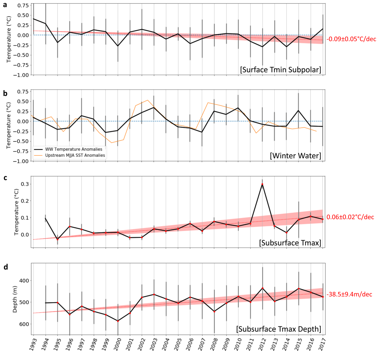
Fig. 4 Time-series of temperature and characteristics of specific water masses. a Zone [B] anomalies, restricted to the gridpoints where the 25 years-mean temperature transect < 0 . b Black line is the WW temperature anomalies from SURVOSTRAL XBTs between 54 and 61.5°S, restricted to the Tmin gridpoints where the 25 year-mean temperature transect is less than 2 °C. Yellow line is the MJJA SST anomalies upstream of SURVOSTRAL WW, between (120–145°E and 57–61°S). c CDW maximum temperature evolution (see “Methods”). Red dots are the years the linear trend is computed on; i.e., years when there is at least 2 months with data on average for each grid point for NDJF months. d CDW maximum temperature depth (see “Methods”). Errors bars are the standard deviation of the mean temperature anomalies (depth for panel d ) for each grid point within the zone.
