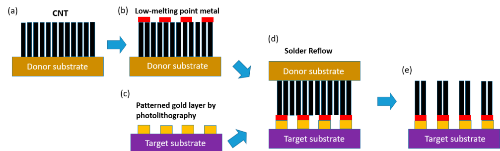
Figure 2. Schematic of CNT transfer method: (a) vertically-aligned CNT growth; (b) evaporation of low-melting point metal such as solder through hard mask onto CNT array; (c) preparation of target substrate; (d) solder reflow process to bond the CNT array and target substrate; (e) separation of CNT array from donor substrate.
