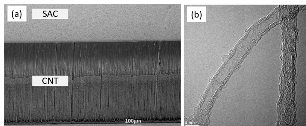
Figure 1. (a) Silver-copper alloy (SAC) deposited on vertically-aligned carbon nanotube (VACNT) does not affect the alignment of the array; (b) Transmission electron microscopy (TEM) image of as-grown CNT.
