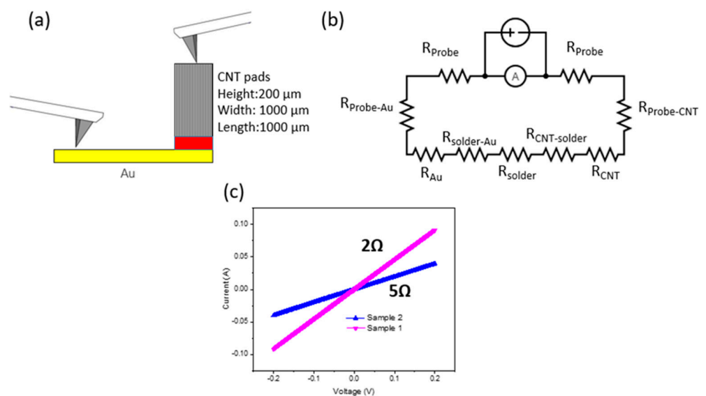
Figure 4. (a) Measurement setup to measure IV-response of transferred CNT array at given CNT dimension; (b) schematic of electrical connection in measurement setup; (c) measured IV-responses and corresponding resistances.
