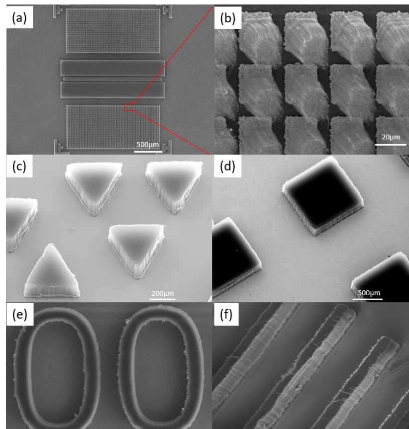
Figure 3. (a,b) Transferred CNT with bump size of 25 μm and a pitch of 10 μm with surrounding bumps; (c–f) multiple shapes of transferred CNT—for (e,f) the width of the CNTs patterns are 200 μm and the height of the CNT 500 μm.
