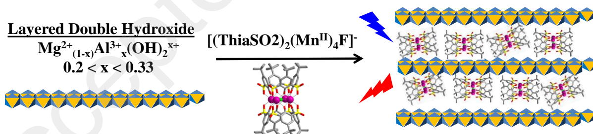
Figure 1: Schematic representation of ThiaSO 2 /Mn II system intercalated in a layered double hydroxide.
