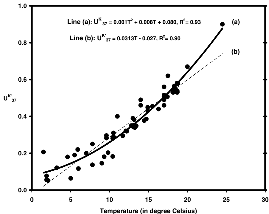
Figure 6. Plot of the water column suspended particles from the Pacific Ocean [Prahl and Wakeham, 1987], Mediterranean Sea [Ternois et al., 1997], Southern Ocean [Sikes and Volkman, 1993] and this study. Line a represents second order polynomial fit of the data; line b is linear fit on the same data set.
