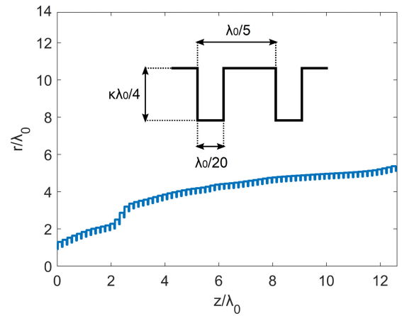
FIGURE 10. Corrugated profile of the TM_{02} launcher. Inset: Dimensions of the used corrugations in terms of wavelength. \kappa corresponds to the correction factor found in [29].
