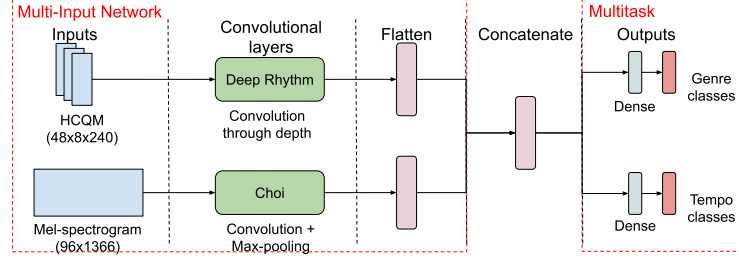
Fig. 2. Architecture for [left] multi-input, [right] multitask.
