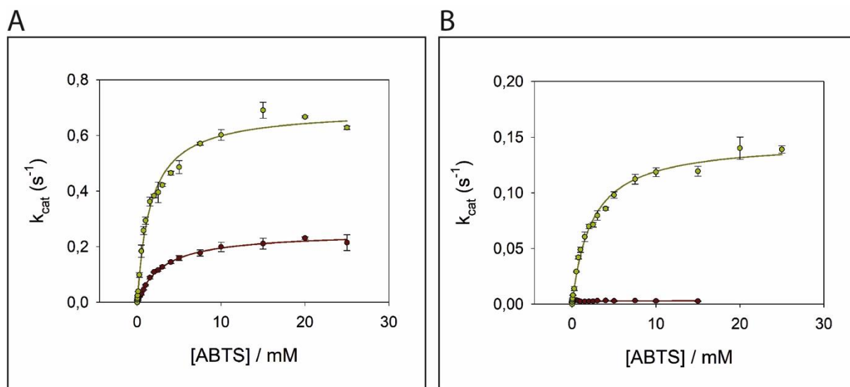
Fig. 7. WT (A) and M456A mutant (B) activity with ABTS, with (dark yellow circles and lines) and without (dark red circles and lines) \text{Cu}^{2+} addition ( 500 \mu\text{M} ) in acetate buffer 50 \text{ mM} at \text{pH} 5.
