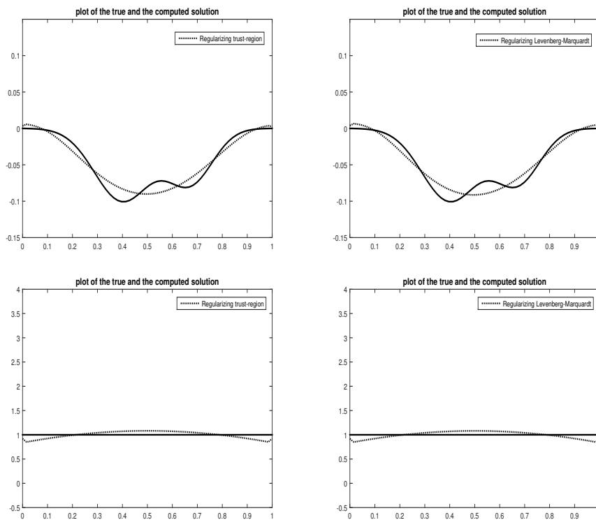
Fig. 3 Regularizing trust-region (left) and regularizing Levenberg-Marquardt (right), true solution (solid line) and approximate solutions (dotted line). Upper part: P1, \delta = 10^{-2} , x_0 = 0e ; lower part: P3, \delta = 10^{-2} , x_0 = x_0(\alpha) = x_0(1.25) .
