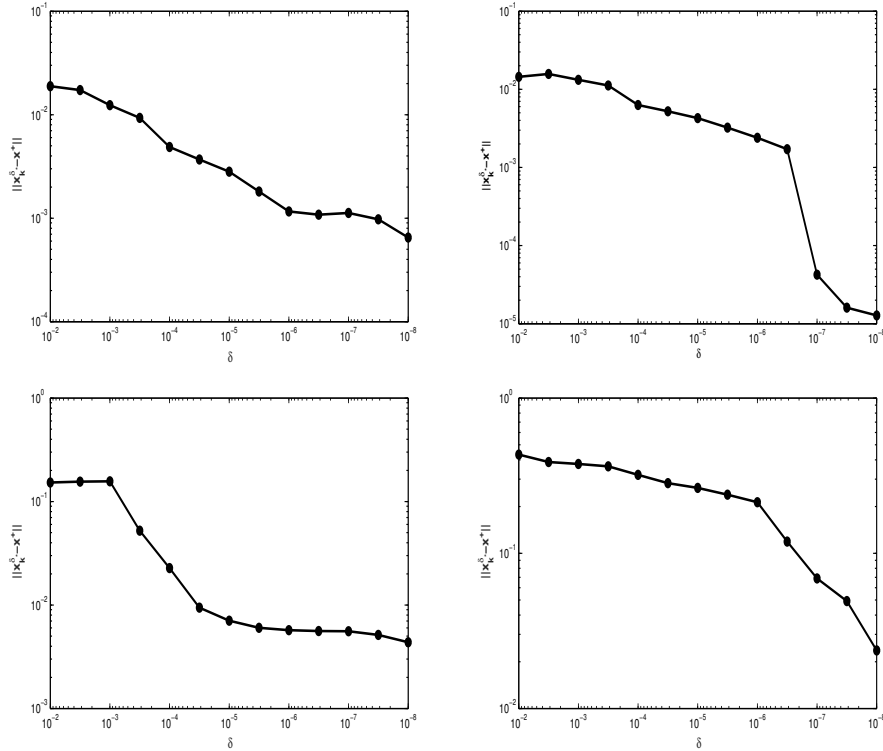
Fig. 2 Regularizing trust-region applied to P1, x_0 = 0e (top left), P2, x_0 = 0e (top right), P3, x_0 = x_0(\alpha) = x_0(1.25) (lower left) and to P4, x_0 = x_0(\beta, \chi) = x_0(0.5, 0) (lower right): log plot of the error \|x_{k^*}^\delta - x^\dagger\| versus the noise \delta .
