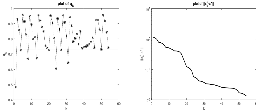
Fig. 1 Regularizing trust-region applied to P2, x_0 = 0e , \delta = 10^{-4} : values q_k = \frac{\|F(x_k^\delta) - y^\delta + J(x_k^\delta)p_k\|}{\|F(x_k^\delta) - y^\delta\|} (marked by an asterisk) and value of q = 1.1/\tau (solid line) versus the iterations (on the left); semilog plot of the error \|x_k^\delta - x^\dagger\| versus the iterations (on the right).
