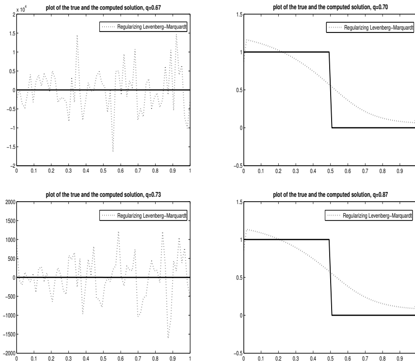
Fig. 5 Problem P4, \delta = 10^{-2} , x_0 = x_0(\beta, \chi) = x_0(1.5, 0) : true solution (solid line) and approximate solution (dotted line) computed by the regularizing Levenberg-Marquardt method for values of q = 0.67, 0.70, 0.73, 0.87 .
