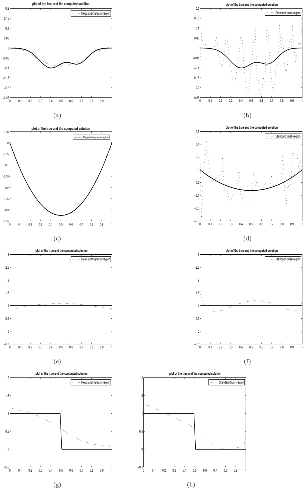
Fig. 6 True solution (solid line) and approximate solutions (dotted line) computed by the regularizing trust-region method (on the left) and the standard trust-region method (on the right). (a)-(b) problem P1, \delta = 10^{-2} , x_0 = 0e ; (c)-(d) problem P2, \delta = 10^{-2} , x_0 = 0e ; (e)-(f) problem P3, \delta = 10^{-2} , x_0 = x_0(1.25) ; (g)-(h) problem P4, \delta = 10^{-2} , x_0 = x_0(0.5, 0) .
