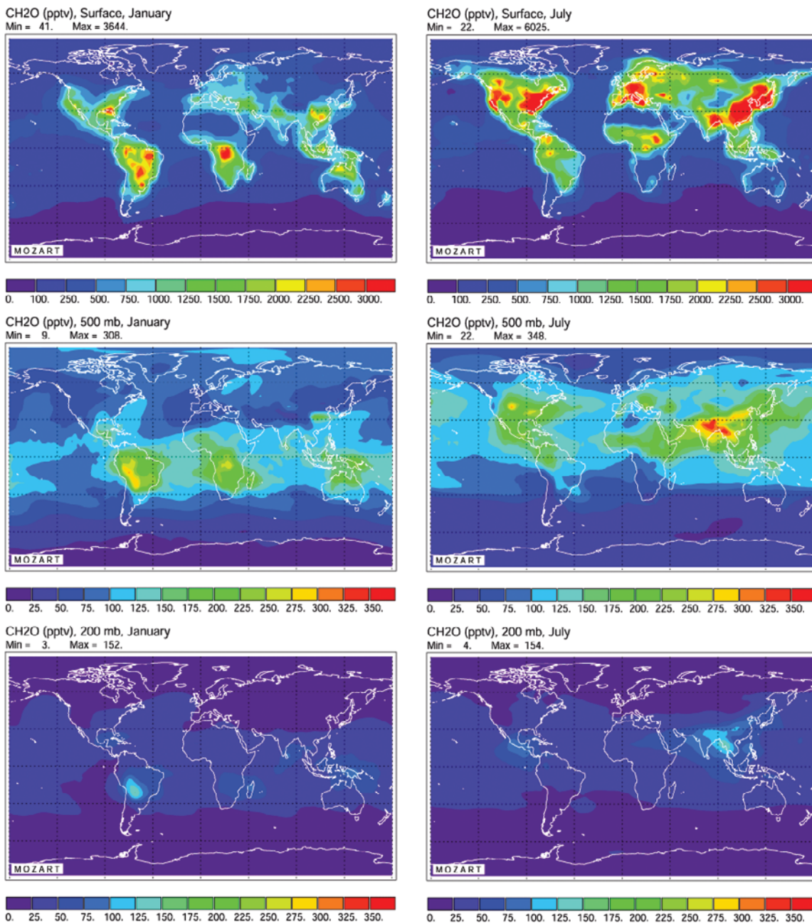
Figure 2. Distribution of CH 2 O calculated at the surface, 500 mb, and 200 mb for January and July conditions (pptv).
