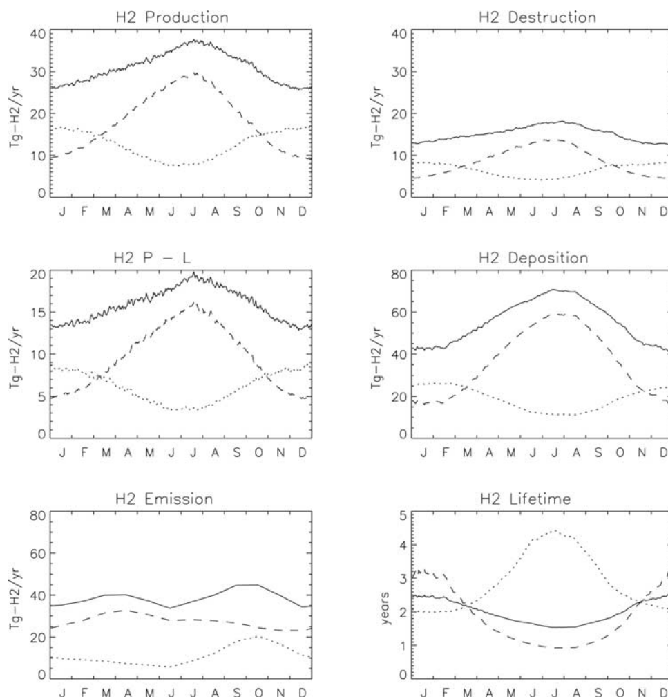
Figure 3. Seasonal variation of integrated \text{H}_2 photochemical production, destruction, and net production ( \text{Tg}/\text{yr} ), surface dry deposition, and surface emission ( \text{Tg}/\text{yr} ), and atmospheric lifetime ( \text{yr} ) calculated by the model. The northern hemisphere values are represented by the dashed line, southern hemisphere is the dotted line, and the solid line is the global integral.
