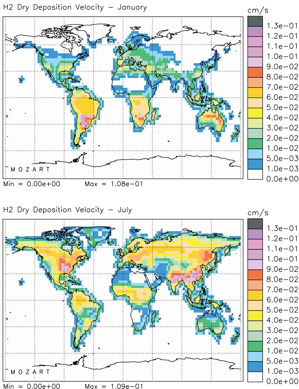
Figure 5. Monthly mean H 2 surface dry deposition velocity (cm/s) considered in MOZART for January and July conditions.
