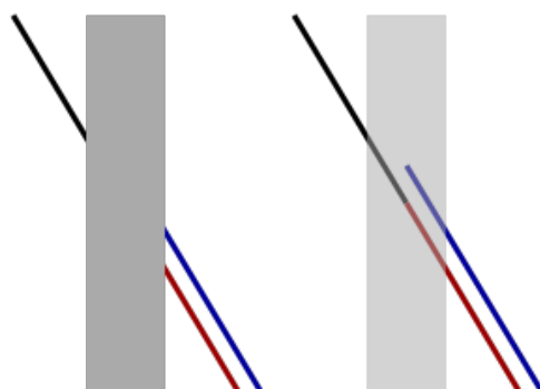
Figure 2. The original Poggendorff illusion: the red colored line is aligned with the black line although the blue one is falsely perceived as its continuation. Source: Wikipedia.
