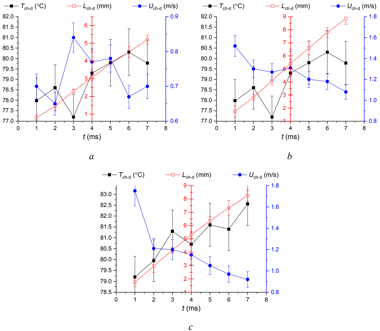
Fig. 19. Temporal variation of the average temperatures ( T_{\text{ch-d}} ), velocities ( U_{\text{ch-d}} ), and distances ( L_{\text{ch-d}} ) of child droplets from the substrate during the destruction of immiscible two-component droplets in the Explosion regime for T_{\text{surf}} \approx 450 °C: a – for droplets with R_{\text{ch-d}} = 0.02\text{--}0.03 mm; b – for droplets with R_{\text{ch-d}} = 0.03\text{--}0.08 mm; c – for droplets with R_{\text{ch-d}} = 0.08\text{--}0.2 mm.
