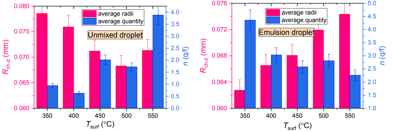
Fig. 14. Average size and number of child droplets resulting from the micro-explosion of emulsion droplets and immiscible two-component droplets with varying temperature surface ( T_{\text{surf}} ) obtained using schlieren photography.
