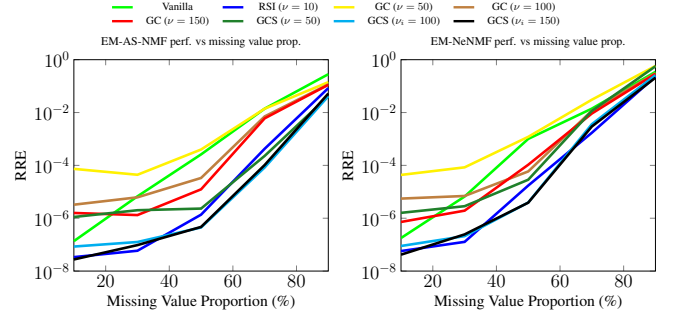
Fig. 3. WNMF performance vs the missing value proportion.
