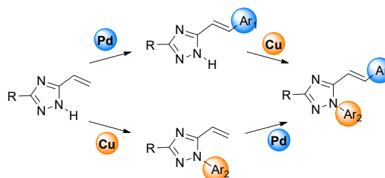
Scheme 1. Selective Pd- and Cu-arylation of 5-vinyl-1,2,4-triazoles.
