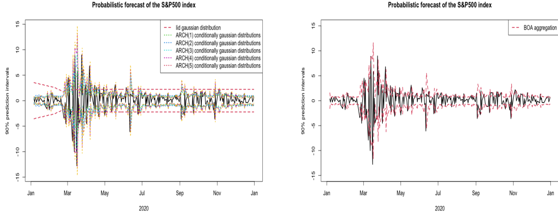
Figure 3: 90%-prediction intervals from 6 forecasters (left) and their BOA aggregation (right).
