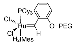
Figure 3. Intermediate complex 12 observed by ^1\text{H} NMR.
