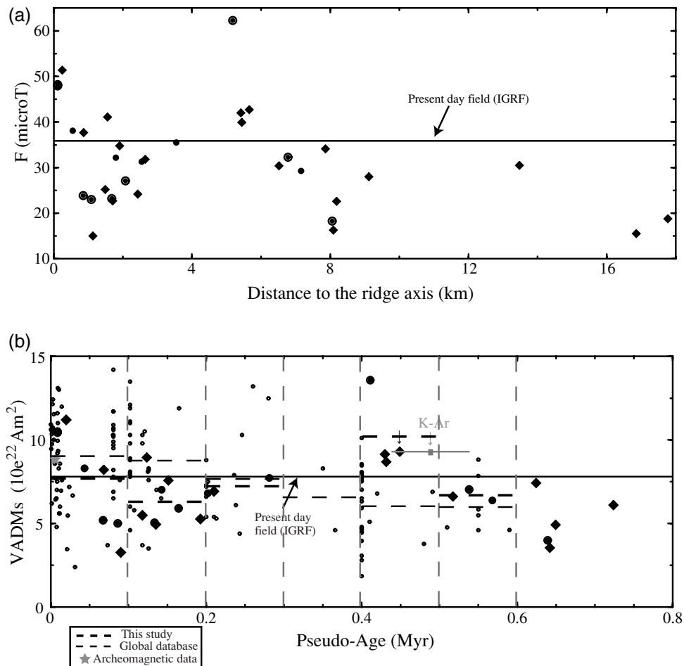
Figure 12. (a) Accurate palaeofield intensities calculated using Tammar materials as a function of the distance to the ridge axis. See Fig. 11(a) for symbols. The present-day field intensity computed at the site by the IGRF is also indicated (black line). (b) Calculated Tammar VADMs for Brunhes chron and selected VDMs extracted from the palaeomagnetic database (small open circles) as a function of the relative age. For comparison, the present-day field intensity computed at the site by the IGRF (black thin line), the mean field intensity for the last 10 kyr given by archaeomagnetic data (grey star) and the mean field intensity calculated each 100 kyr using Tammar samples and the global database (thick and thin dashed lines, respectively) are indicated. The grey line indicates the absolute K–Ar age of sample 103.
