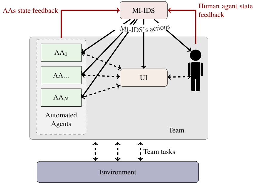
Fig. 1. Mixed-Initiative Interaction Driving System (MI-IDS) architecture. UI: User Interface.
