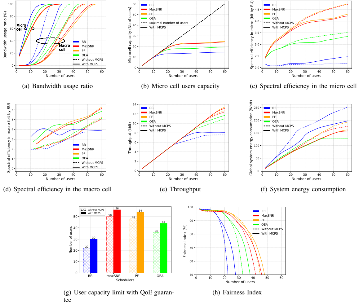
Figure 12: Performance results for scenario 1
