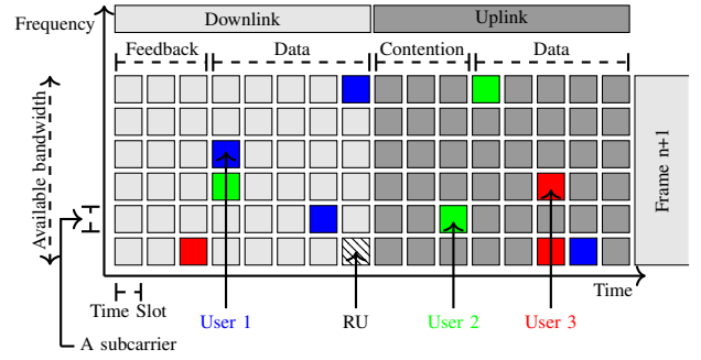
Figure 3: 5G frame structure in TDD mode
