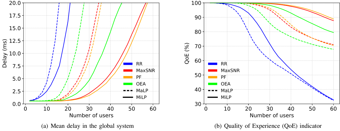
Figure 5: MiLP/MaLP performance results comparison
