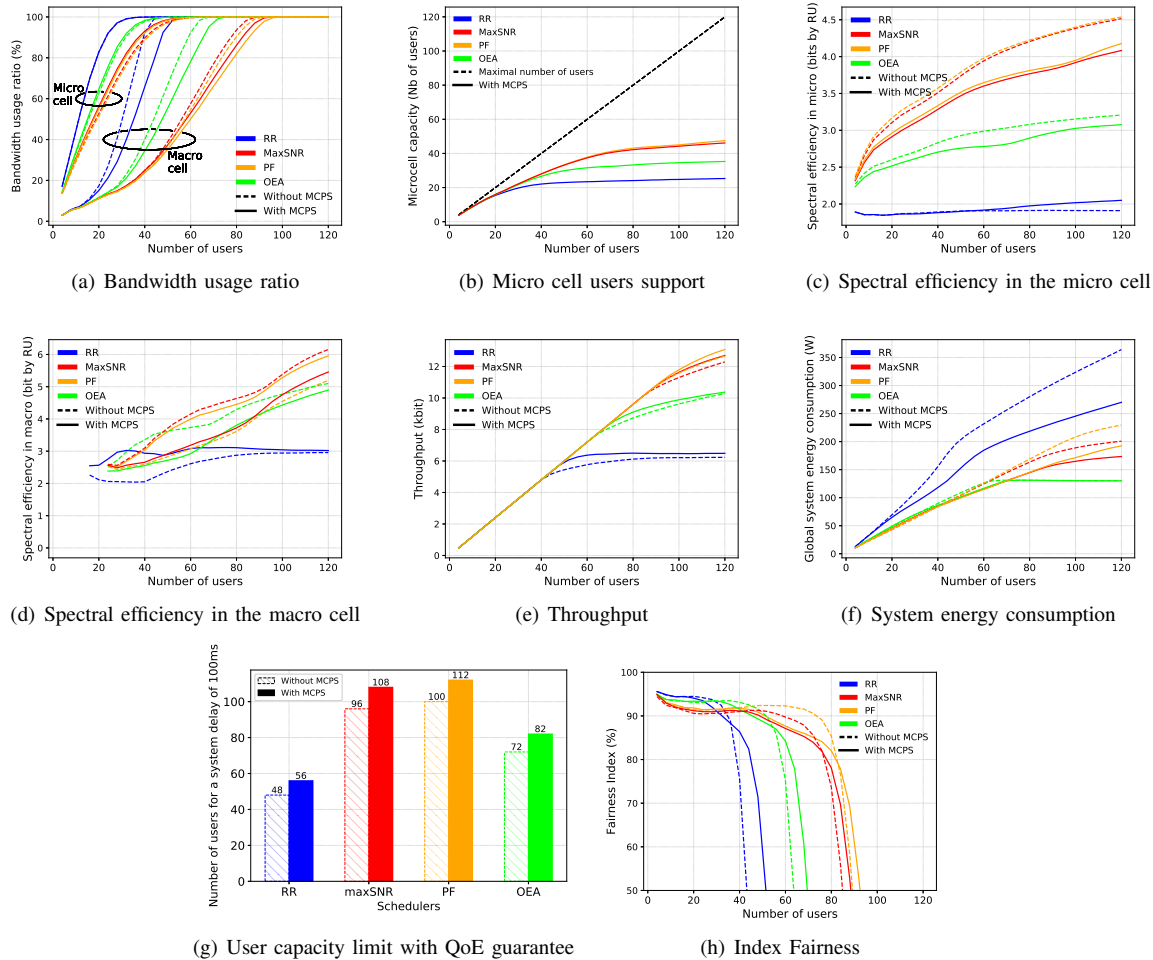
Figure 13: Performance results for scenario 2
