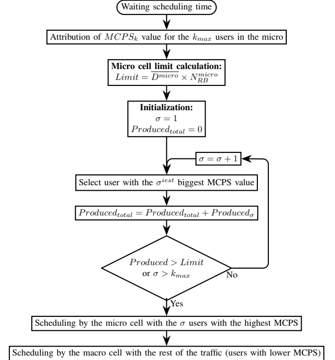
Figure 7: MCPS pre-scheduler algorithm flow chart
