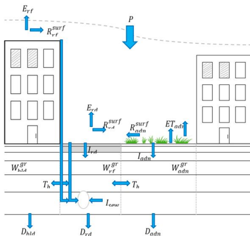
Figure 1 : Diagram of the hydrological processes modelled in the TEB-Hydro model; subscripts rf and bld stand for building compartment, rd for road compartment and gdn for garden compartment. (Stavropoulos-Laffaille et al., 2018)
