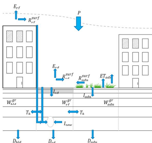
Figure 1 : Diagram of the hydrological processes modelled in the TEB-Hydro model; subscripts rf and bid stand for building compartment, rd for road compartment and gdn for garden compartment. (Stavropoulos-Laffaille et al., 2018)
