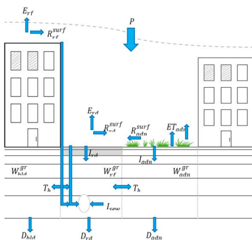
Figure 1 : Diagram of the hydrological processes modelled in the TEB-Hydro model; subscripts rf and blt stand for building compartment, rd for road compartment and gdn for garden compartment. (Stavropoulos-Laffaille et al., 2018)
