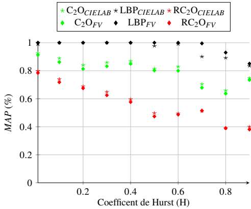
(b) MAP per Hurst coefficient
