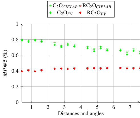
(a) Mean P@5 for each distances and angles
