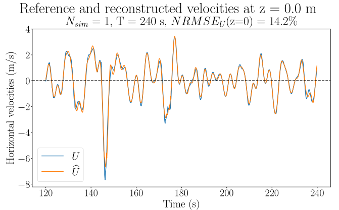
Fig. 6. Extract of a reconstructed velocity time series at z = 0 for \epsilon_c = 3.5\% ( H_s = 7.82\text{m} ). The NRMS error on U computed on these 240 s is comparable to the converged error value. Hence, the time series is a good illustration of what can be expected in terms of velocity reconstruction.
