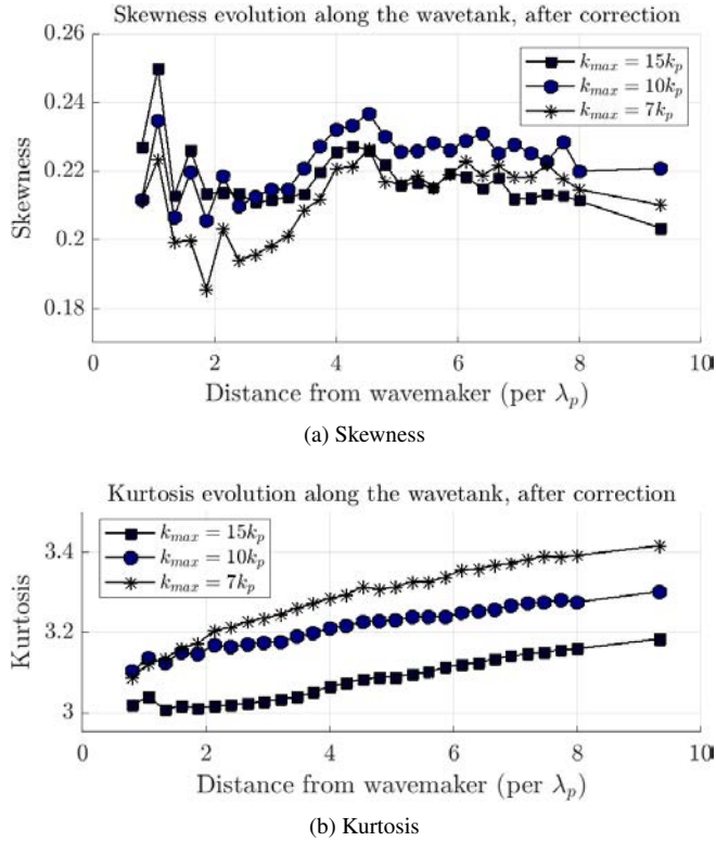
FIGURE 13: CASE 3 STATISTICAL QUANTITIES ALONG WAVETANK - X_t = 1.9\lambda_p .
