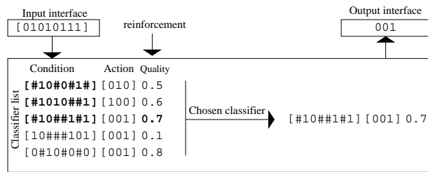
Fig. 3 In a strength-based LCS, classifiers are composed of a [Condition] part, an [Action] part, and a value that is both the classifier fitness and its estimation of expected reward. Among the classifiers, the system selects those whose [Condition] part matches the current situation and chooses one classifier in that set with a roulette wheel mechanism. The corresponding action is executed (in the example, the agent executes [001]).
