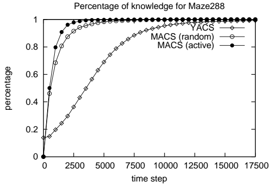
Figure 16: Evolution of the percentage of knowledge in Maze288
