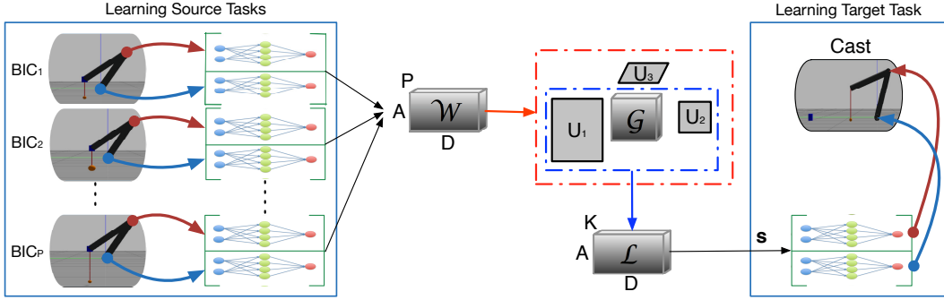
Figure 2: Transfer Learning Schematic. A set of P source tasks are learned and the matrices representing each source policy are stacked into a tensor \mathcal{W} . Factorising \mathcal{W} separates task-specific, actuator-specific and shared knowledge. Task-independent latent skills are gathered in tensor \mathcal{L} . For the target task, the agent learns the weights \mathbf{s} that reconstructs \mathcal{L} into policy parameters.
