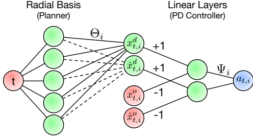
Figure 1: Network defining our policy \mathbf{a}_i = \pi(\mathbf{x}_{t,i}^o, t) from time-step t and observed state \mathbf{x}_{t,1}^o to action a_{t,i} .
