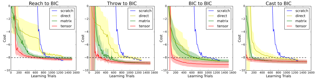
(a) Learning curves of transfer learning from 4 source tasks to BIC tasks
