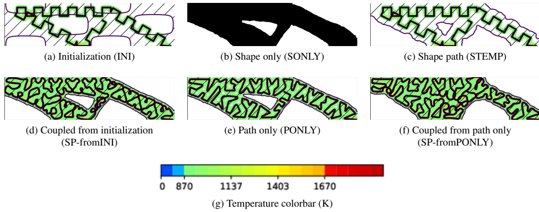
Figure 22: Initialization and shape optimization for different tests, initialization 2, aluminium, half large cantilever, V^{\text{target}} = 1.1V^0
