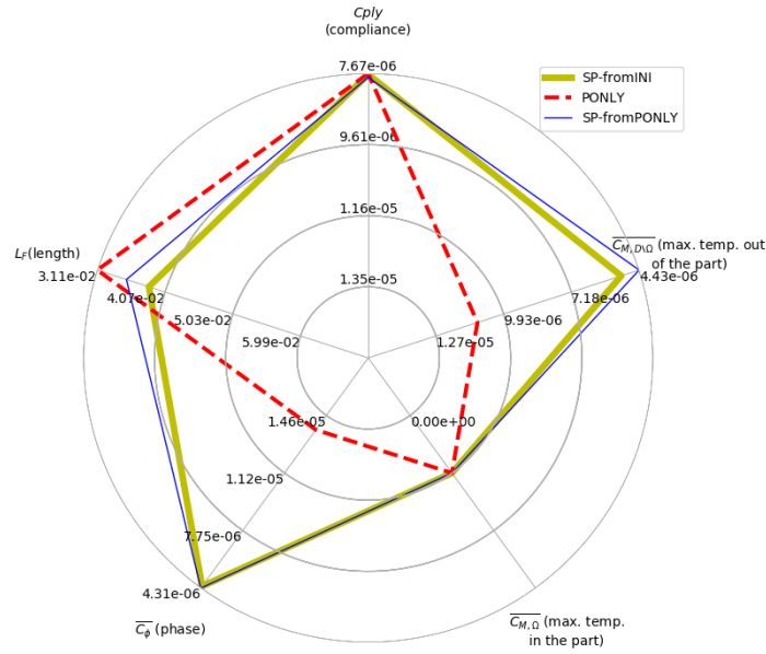
Figure 21: Radar chart of the values given in Table 11, initialization 1, aluminium, half large cantilever, V^{\text{target}} = 1.1V^0
