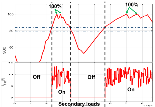
Fig. 8 SOC and secondary loads current variation during scenario 3 (secondary loads connection / disconnection SOC's set at 85% / 80% respectively)
