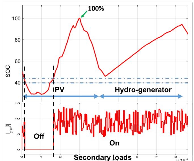
Fig. 10 SOC and secondary loads current variation during scenario 3 (secondary loads connection / disconnection SOC's set at 45% / 40% respectively)
