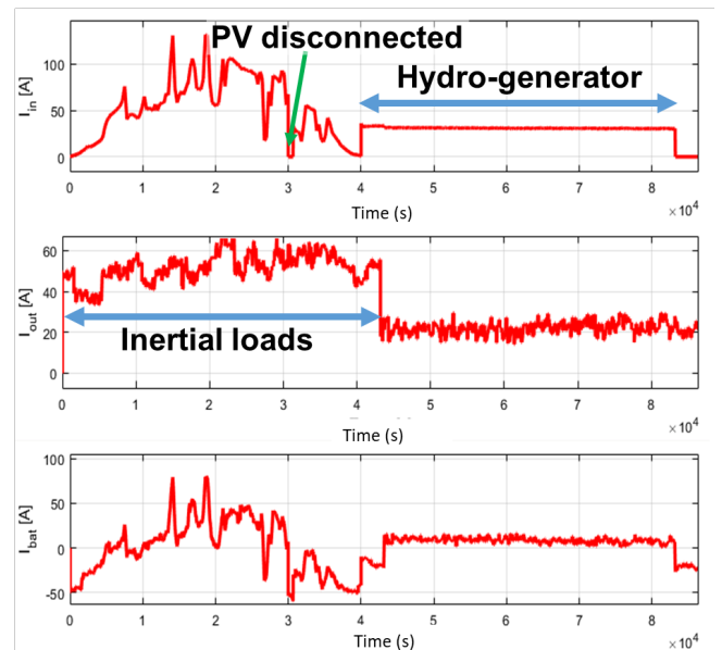
Fig. 11 Charger currents variation during scenario 3 (secondary loads connection / disconnection SOC's set at 45% / 40% respectively)
