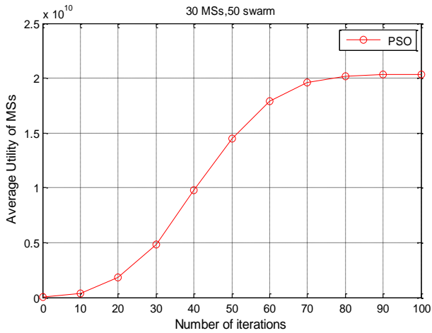
Figure 3: Convergence of PSO iterative algorithm
